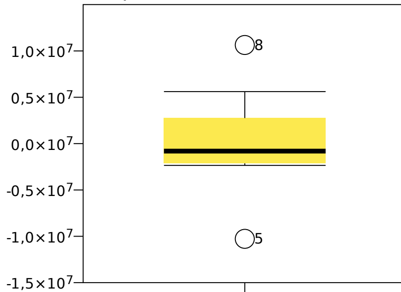
Boxplot of RES1
