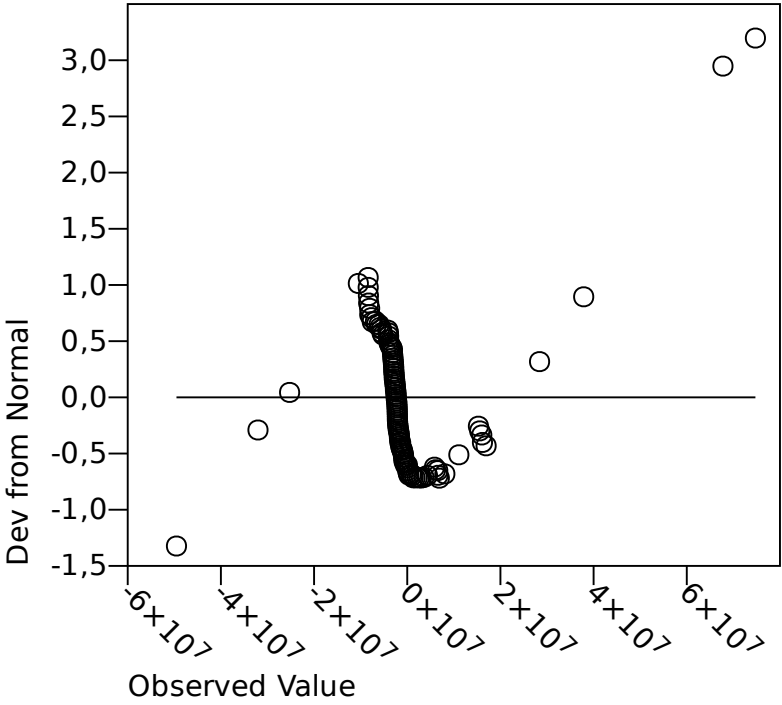
Detrended Normal Q-Q Plot of RES1
