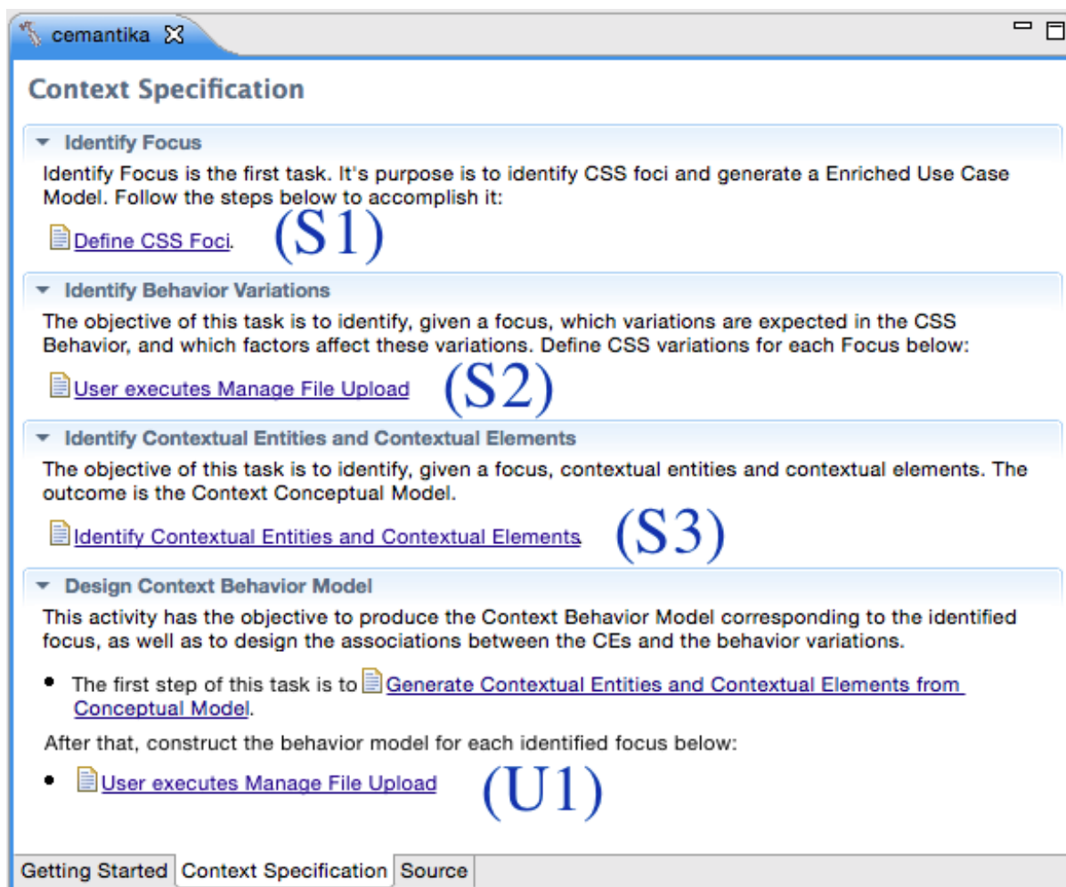
Figura 2.11 CEManTIKA Modeling (Patricio, 2010)
