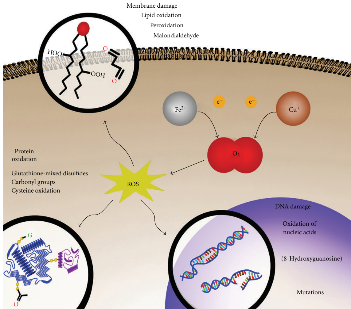
FIGURE 2: Oxidative damages induced by transition metals. Iron and copper can reduce oxygen leading to ROS generation and subsequent oxidation of proteins, lipids, and nucleic acids.
