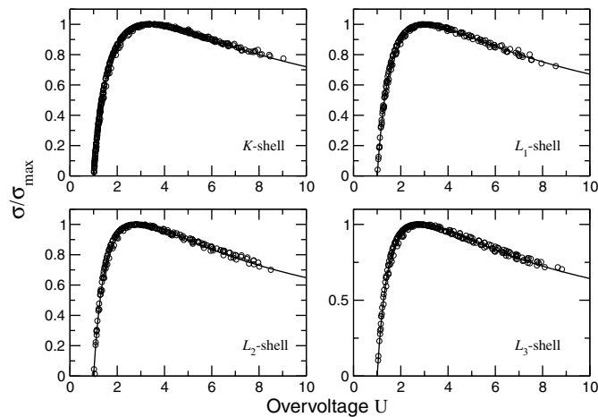
Figure 1. Overvoltage dependence of the calculated ionization cross sections by the DWBA method [12], normalized to the maximum height, for (a) K , (b) L 1 , (c) L 2 and (d) L 3 atomic shells. The continuous curve is the result from the analytical expression proposed in this work. The symbols represent DWBA calculations of Be, B, C, O, F, Al, Si, S, K, Ti, Cr, Mn, Fe, Ni, Cu, Ge and Zr for the K -shell, and of Ni, Cu, Ge, Zr, Ag, Te, W, Pt and Au for the L 1,2,3 -subshells.
