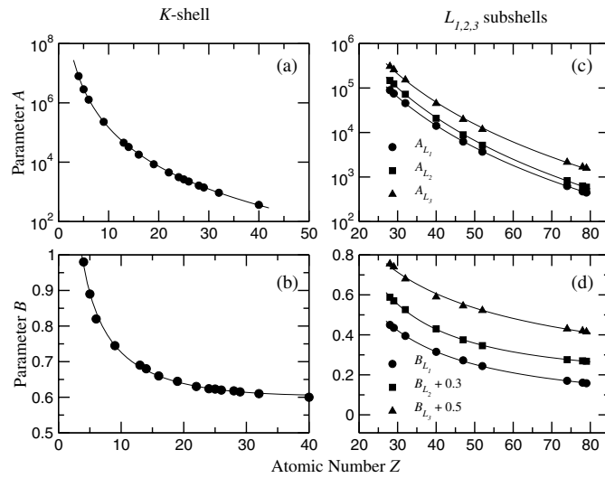
Figure 2. Variation of the parameters A and B with atomic number, given in equation (2) to describe the absolute ionization cross section values obtained by the DWBA method [12]. (a) Parameter A for K -shell. (b) Parameter B for K -shell. (c) Parameter A for L_1 , L_2 and L_3 -subshells. (d) Parameter B for L_1 , L_2 and L_3 -subshells. The continuous lines correspond to the functions fitted for each parameter given in table 1.
