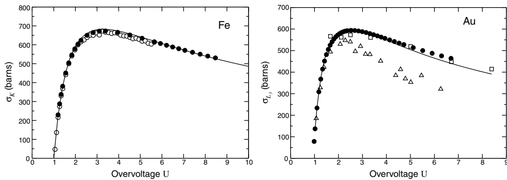
Figure 3. Total cross sections for ionization of the K -shell of iron and the L_3 -shell of gold. The solid line represents the results obtained by equation (2) proposed in this work. The DWBA results are represented with solid circles [12]; the open symbols represent experimental data: circles [15], squares [20], triangles [21].
