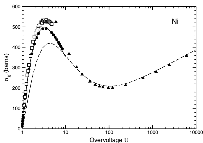
Figure 4. Total cross section for ionization of the K -shell of nickel obtained using the DWBA method (solid circles) [12], the model proposed by Mayol and Salvat [7] (dashed line) and calculations by Scofield [6] (triangles). The open symbols are experimental data [14]. The solid line represents the results obtained with equation (2) proposed in this work.
