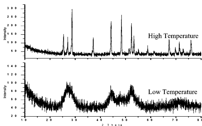
Figure 1. X-ray diffraction patterns of comparing the high-temperature, hexagonal phase CdS (hex-CdS) to the thermodynamically favored cubic crystalline bulk-phase CdS (c-CdS).
