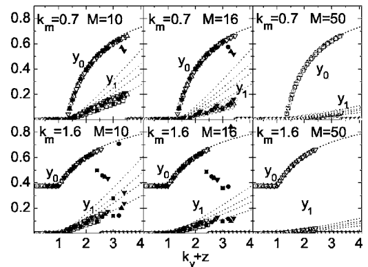
FIG. 2. Solutions y_0 and y_1 : Simulation results for finite M=10 and 16 (solid symbols); theoretical solutions for M=10, M=16 , and M=50 (open symbols); theoretical solution in the M \rightarrow \infty limit (dashed lines). We considered k_v=0.2 (squares), 0.4 (circles), 0.5 (up triangles), and 0.6 (down triangles). Larger k_v yields larger y_1 .
