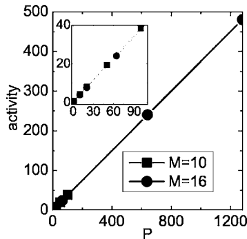
FIG. 5. Global activity a as function of network load P for k_m=1.6 , k_v=0.25 , and z=1.0 , in the presence of a nonzero external noise: a goes linearly with P indicating that all memorized patterns are excited by the external noise. We show results for M=10 and M=16 . The inset shows the linear dependence for initial values of P .
